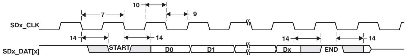
Figure 8-87. MMC/SD/SDIO Host Write Timing
