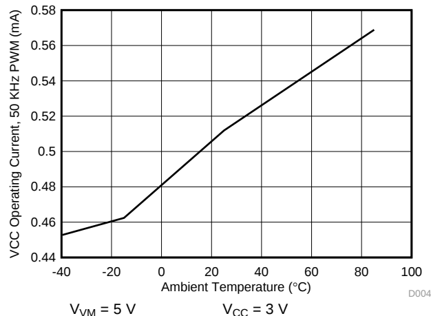
Figure 5. VCC Operating Current vs Ambient Temperature
